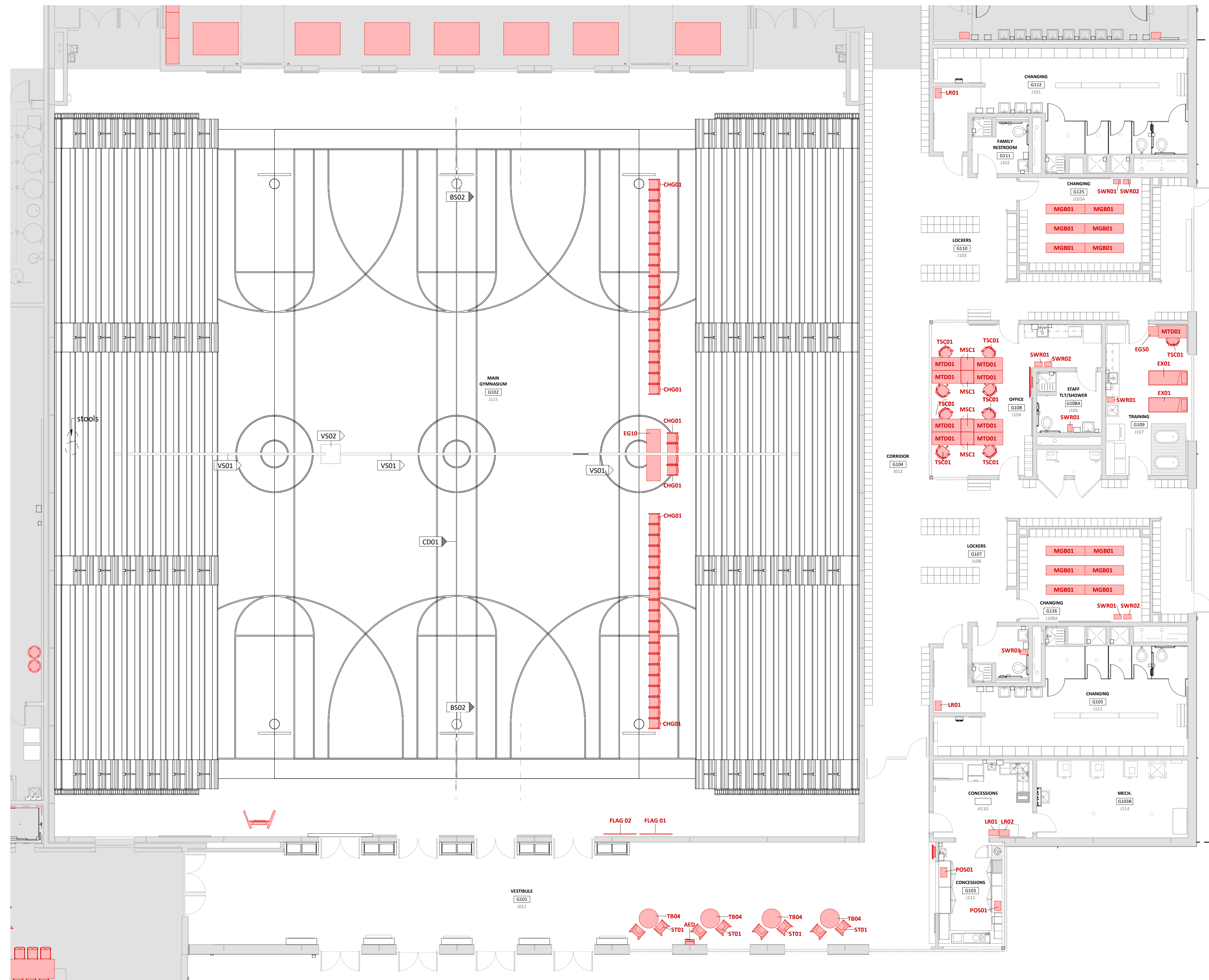
LEVEL 1 FFE PLAN - AREA J ATHLETICS
